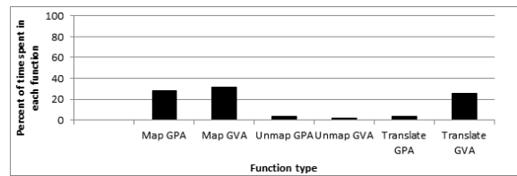
Figure 3: Percent of time spent in memory-mapping routines.
