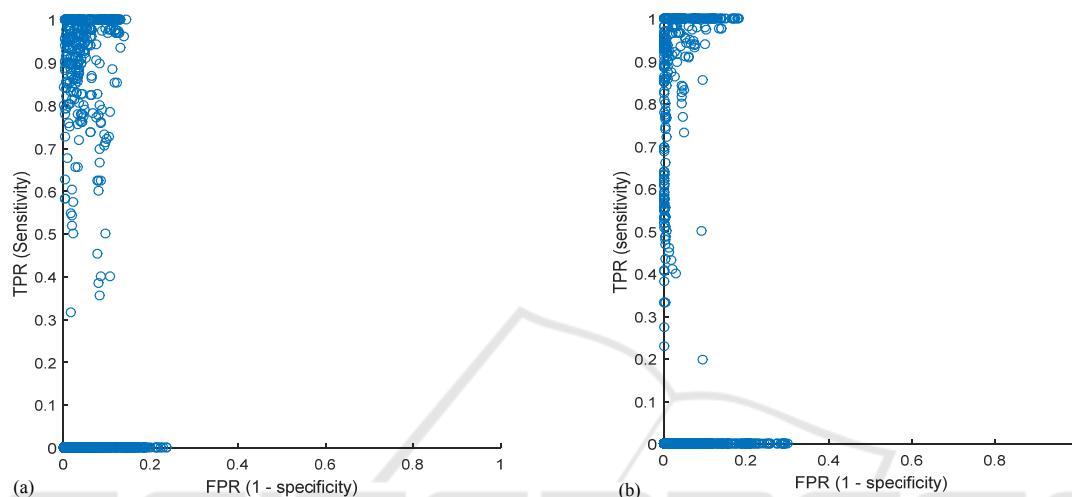
Figure 5: Example of ROC spaces for the scanning sequences. a) ROC space for the graph-based segmentation method with the GLCM energy, b) ROC space for the J-image segmentation with the GLCM energy.
