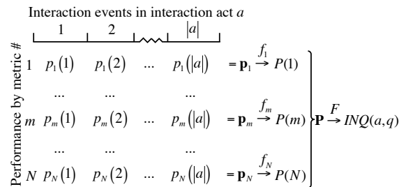
Figure 3: Derivation of interaction quality INQ(a, q) for an interaction act a when performing task q . N metrics are used to compute performance related to both robot and human. Fusion of performance is done first at event, and then at metric level by the functions f_i and F respectively.
