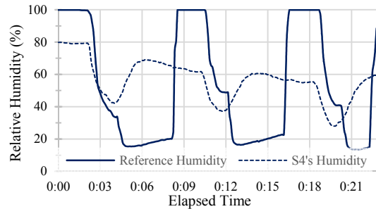
Figure 9: Humidity timeseries from dynamic scenario.
