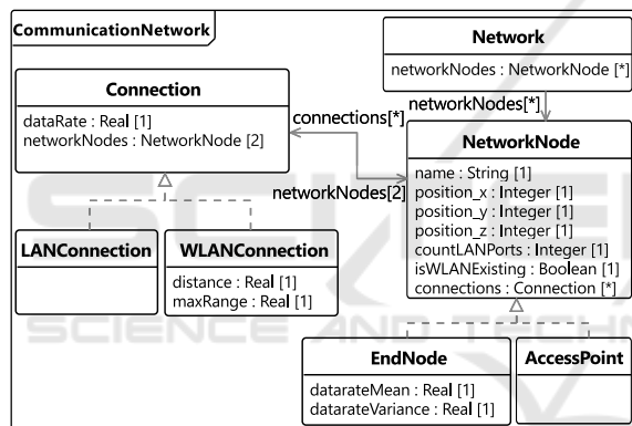
Figure 10: Design of communication network.
