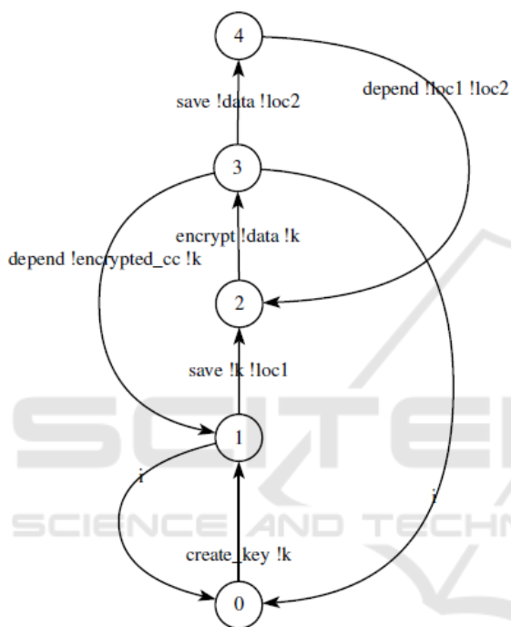
Figure 6: Minimized Labeled Transition System for the sample code given in Figure 1.
