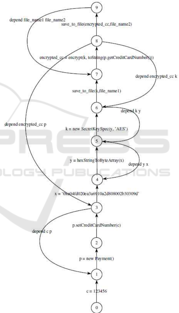
Figure 5: Labeled Transition System for the sample code given in Figure 1.
