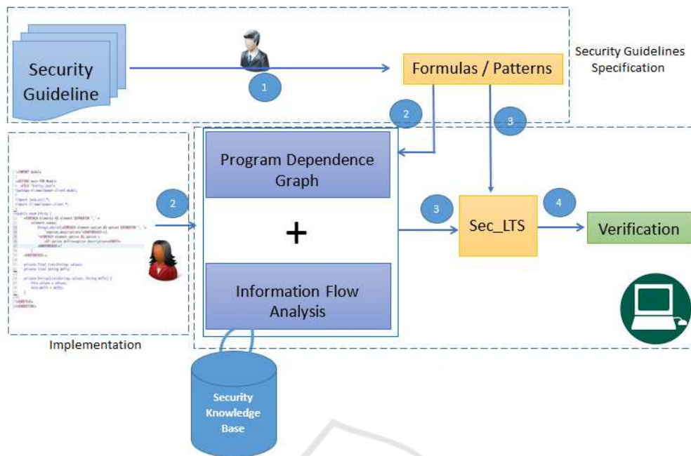
Figure 3: End-to-end Approach.
