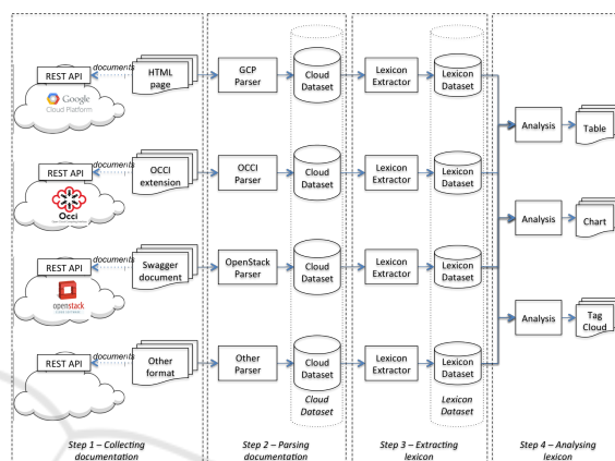
Figure 1: CLOUDLEX Approach.
