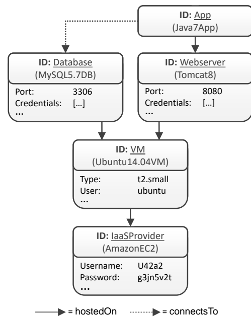
Figure 2: Exemplary TOSCA Topology Template.
