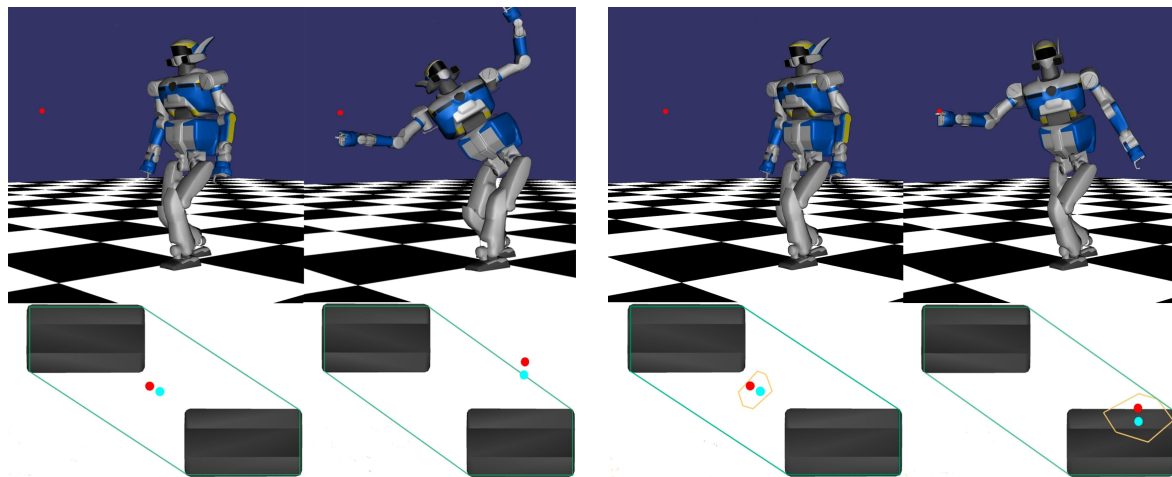
(a) Classic control illustrating the robot’s loss of balance when the real capture point gets out of the support polygon. (b) Robust control illustrating the robot right end effector reaching close to the goal without losing balance.
