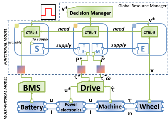
Figure 8: Functional to multi-physical domain interconnection.
