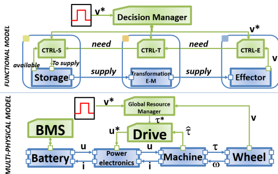
Figure 7: Control system and flow exchange representations of functional and multi-physical modeling.
