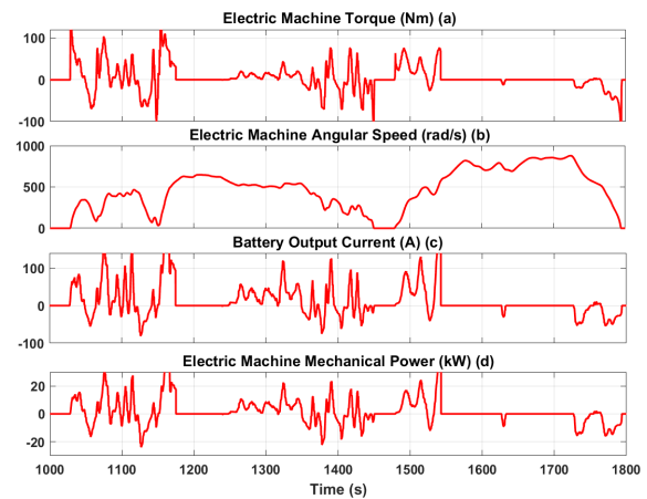
Figure 15: Hybrid vehicle electric machine results.
