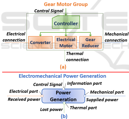
Figure 6: Multi-physical (a) & functional (b) model representations.
