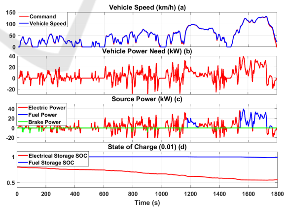
Figure 13: Parallel PHEV - simulation results using the functional model (Mokukcu et al., 2016).
