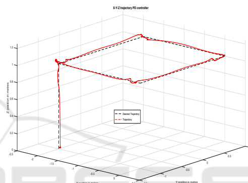
Figure 7: Real 3D trajectories using a PD controllers.
