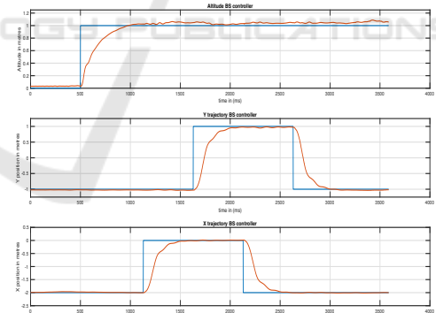
Figure 8: Real XYZ displacement with a BS controllers.
