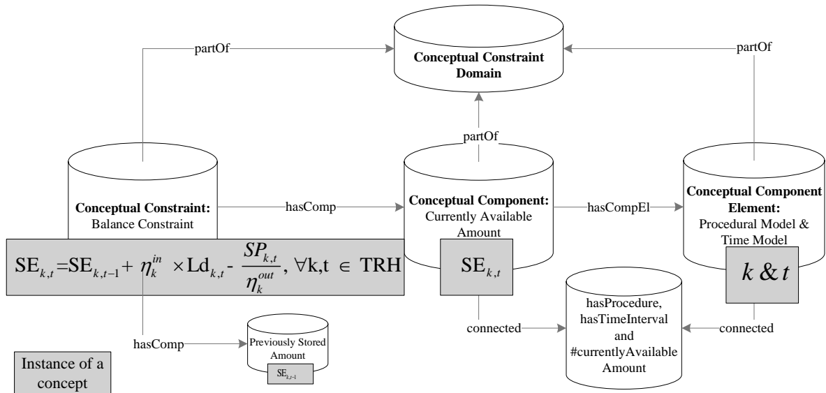
Figure 5: Connections of Conceptual Models with the Example.
