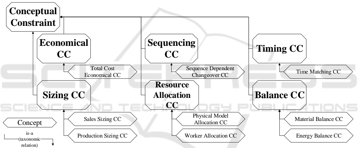
Figure 2: Part of the Conceptual Constraint Taxonomy in the CC Domain.
