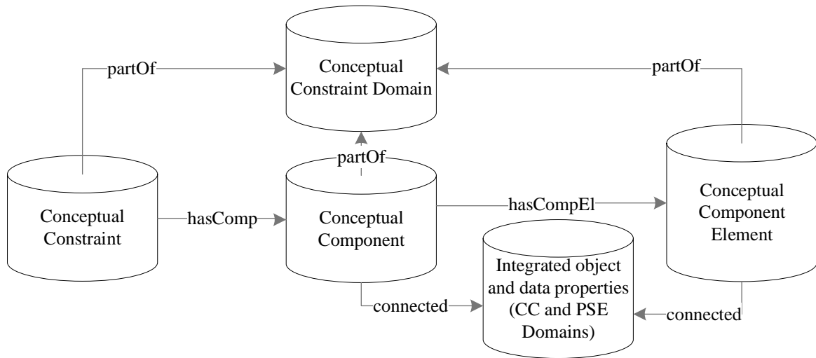
Figure 1: Relations in the CC Domain.
