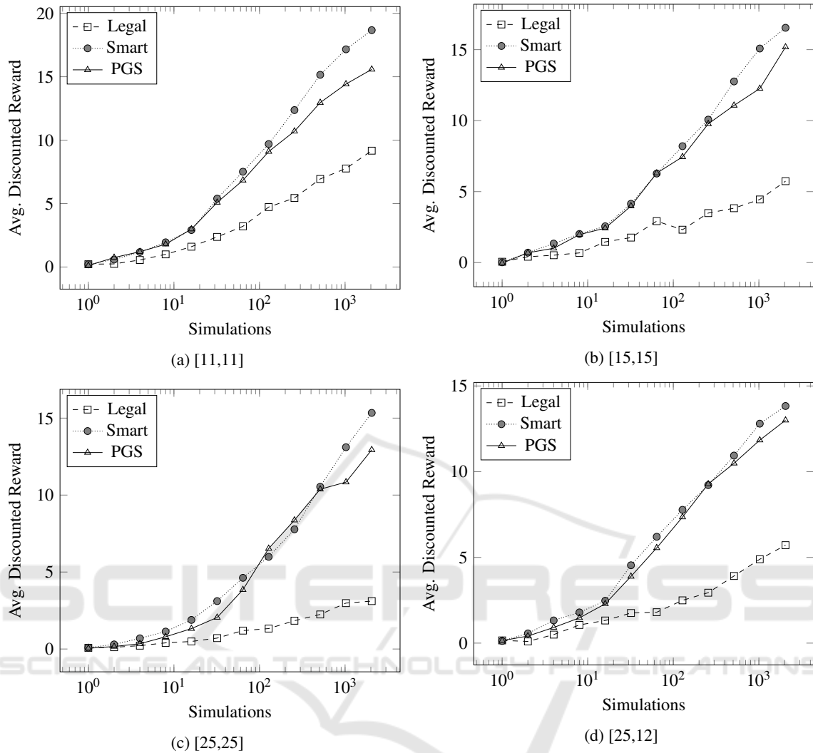
Figure 3: Performance in Rocksample.
