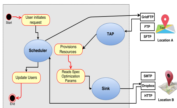
Figure 4: OneDataShare's interoperability components.
