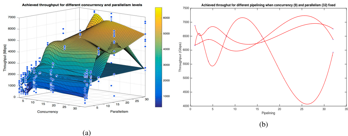
Figure 1: This figure shows the variation in achievable throughput in 10 Gbps XSEDE network between Stampede (TACC) and Gordon (SDSC). Cubic spline surface is constructed to interpolate throughput for the whole parameter space. (a) Shows the impact of concurrency and parallelism parameters on the throughput. The colors represent the throughput in Mbps, blue being the lowest and yellow being the highest throughput. The blue dots represent actual measured throughput values for the corresponding parameters. (b) The impact of pipelining on throughput is demonstrated.
