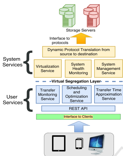
Figure 2: OneDataShare high-level overview.
