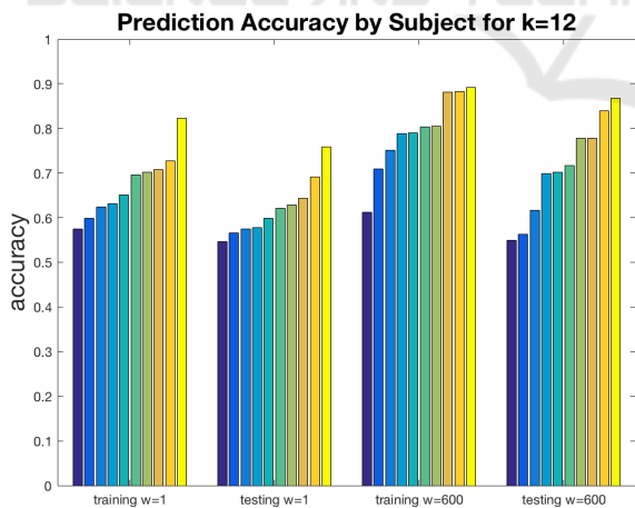
Figure 7: Prediction Accuracy as a function of k in 4-fold cross-validation for k=12
