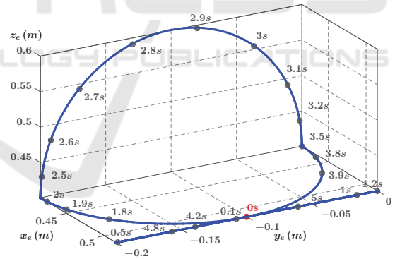
Figure 2: Testing trajectory with specific time marks.
