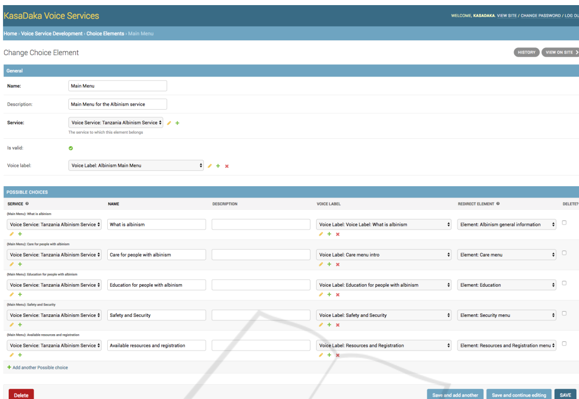
Figure 3: An example screen shot of the voice-service development interface of the VSDK. Shown is an example of a choice interaction element. A voice service developer uses this GUI to develop voice-based applications on the Kasadaka platform.
