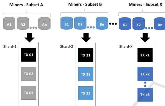
Figure 7: Sharding.
