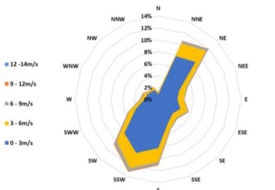
Figure 14: Wind rose in Casablanca
