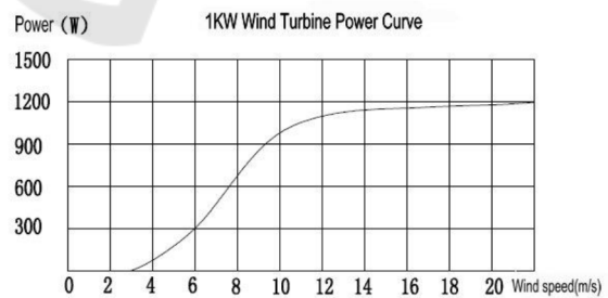
Figure 17: HUMMER 1kW Power / wind speed curve.
