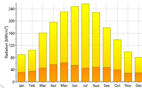
Figure 4: Global (yellow) & Diffuse (orange) radiations in Tangier;
