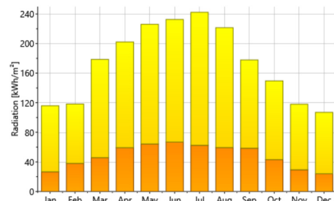
Figure 3: Global (yellow) & Diffuse (orange) radiations in Marrakech;
