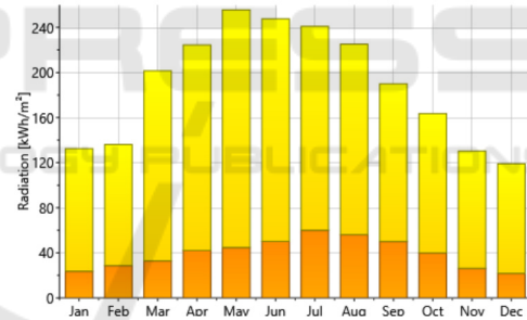
Figure 5: Global (yellow) & Diffuse (orange) radiations in Ouarzazate;
