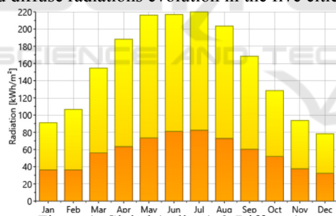
Figure 1: Global (yellow) & Diffuse (orange) radiations in Casablanca;
