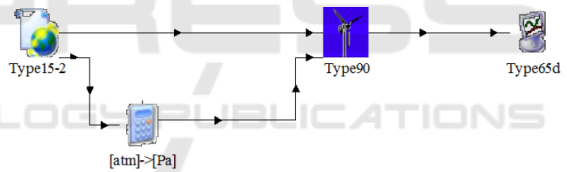
Figure 16: TRNSYS model.
