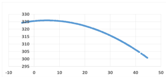
Figure 13: Effect of the temperature on the electrical yield of 1 hour (in Watt)
