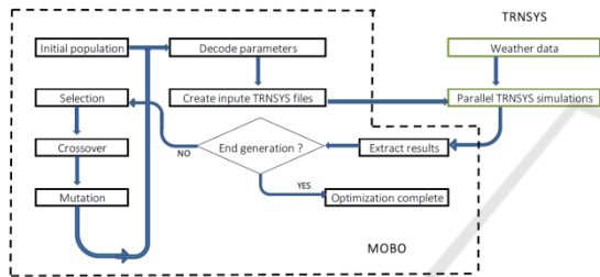
Figure 10: Coupling TRNSYS / MOBO GA
