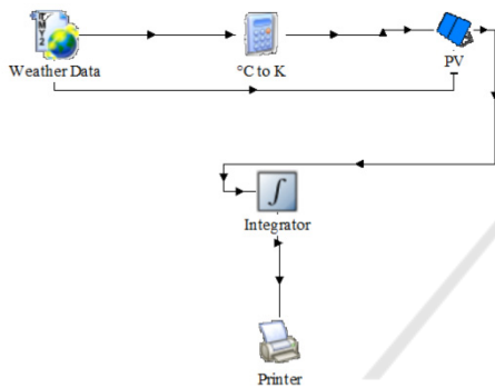
Figure 7: TRNSYS model
