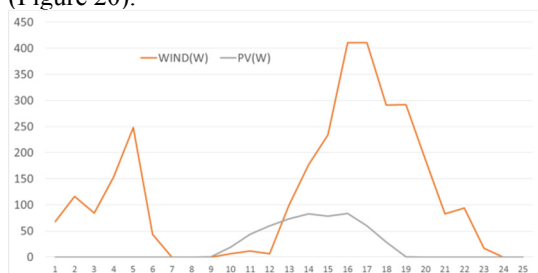
Figure 20: PV and wind yield in the 31th of December
