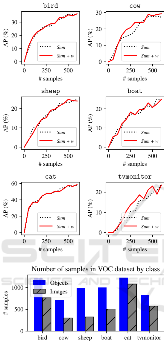
Figure 4: Class-wise validation results on part B of the VOC dataset (i.e., unknown classes). The first row details the first way of splitting (bird,cow,sheep) while the second row shows the second way (boat,cat,tvmonitor). For reference, the distribution of samples (object instances as well as images with at least one instance) over the VOC dataset is provided in the third row.
