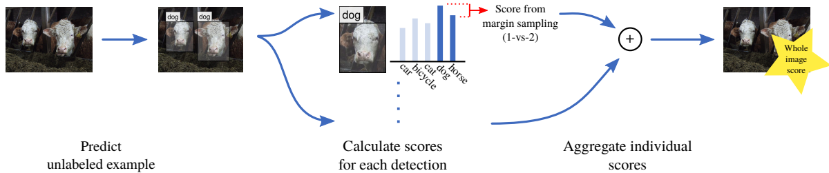
Figure 1: Our proposed system for continuous exploration scenarios. Unlabeled images are evaluated by an deep object detection method. The margins of predictions ( i.e. , absolute difference of highest and second-highest class score) are aggregated to identify valuable instances by combining scores of individual detections.
