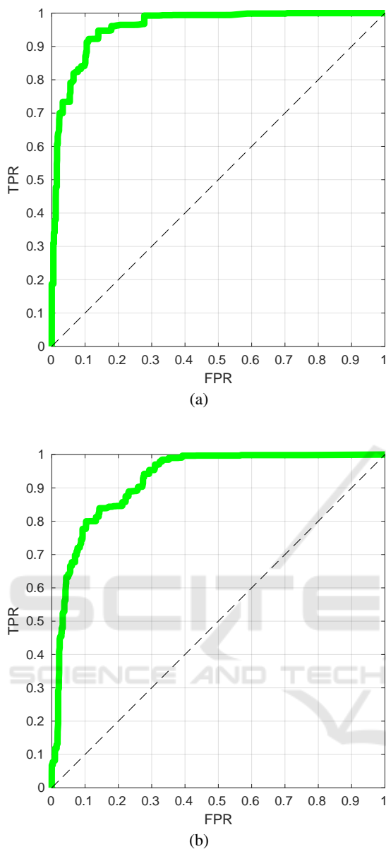
Figure 11: ROC curves obtained from the improved 2D change maps. In (a) ROC for I_0 vs I_1 achieving an AUC of 0.96. In (b) ROC for I_2 vs I_3 achieving an AUC of 0.92.
