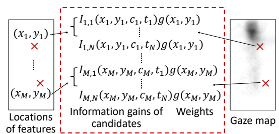
Figure 5: Assigning weights for information gains.
