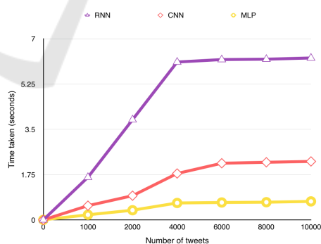
Figure 1: Time taken to perform relevance classification on a collection of Tweets.
