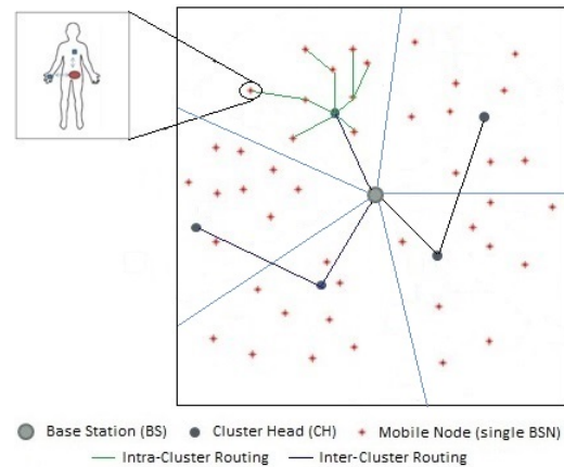
Figure 2: Proposed Algorithm Illustration.
