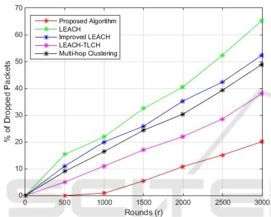
Figure 5: Percentage of Dropped Packets.
