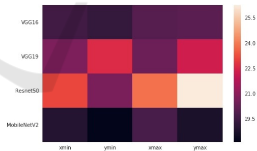
Figure 9: Weights assigned to CNN architectures for prediction of the corners of bounding boxes in localization. xmin and ymin are left bottom coordinates and xmax and ymax are top right coordinates.
