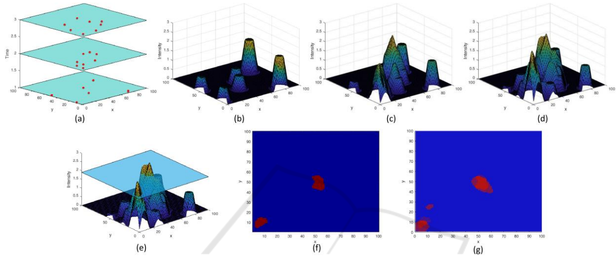
Figure 2: Samples processing phases. Each sample in a given time instant (a) is transformed into a mark (b); each mark aggregates with the marks released in previous time instants and properly “evaporated” (c-d); a threshold is used to identify the areas corresponding to the significant part of the trail (e-f); those areas are compared to measure their similarity (g).
