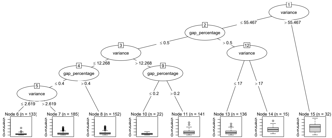
Figure 4: Learned model.
