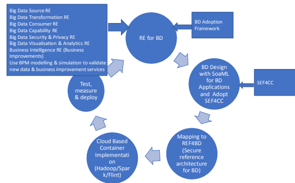
Figure 5: SOSEBD Lifecycle.
