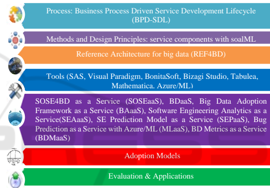
Figure 3: SOSE4BD Framework.
