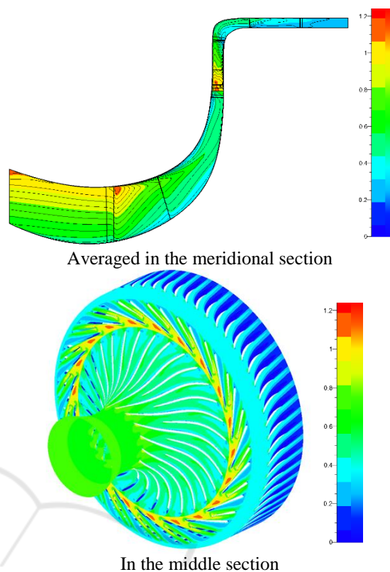
Figure 5: Calculated contours of Mach numbers in the relative motion at the design point, obtained for the compressor using computational 3D model.
