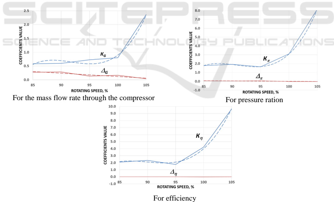
Figure 8: The results of calculating the transformation coefficients in identifying 2D characteristics of a virtual prototype (solid line) and their interpolation (dashed line).
