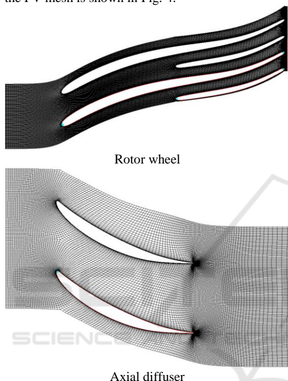
Figure 4: Finite volume mesh of a 3D computational model of the centrifugal compressor.
