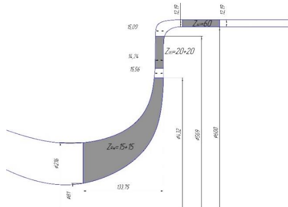
Figure 2: Meridional shape of a centrifugal compressor.
