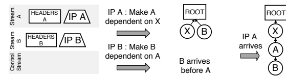
Figure 5: HTTP/3 before draft-22: B ‘steals’ bandwidth from X. (IP: Initial PRIORITY message).
