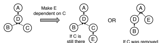
Figure 3: HTTP/2 behaviour when referenced parent does not exist. E is added as a sibling of D on the root, (unintentionally) sharing its bandwidth.
