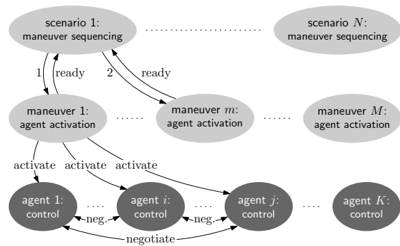
Figure 5: The coordination layer (light gray) and the motion control layer (dark grey) in an agent-based control approach.
