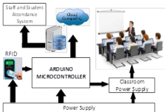
Figure 1: NumberBlock diagram of student attendance system.
