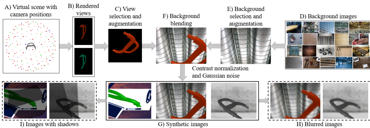
Figure 2: Synthetic dataset generation. Details in Section 3.1.
