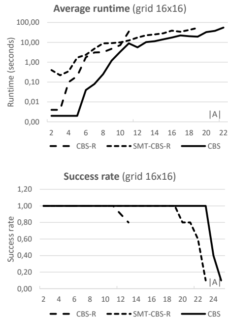
Figure 4: Comparison of CBS R and SMT-CBS R on 16 \times 16 grid with 2^k neighborhood ( k = 3 ).
