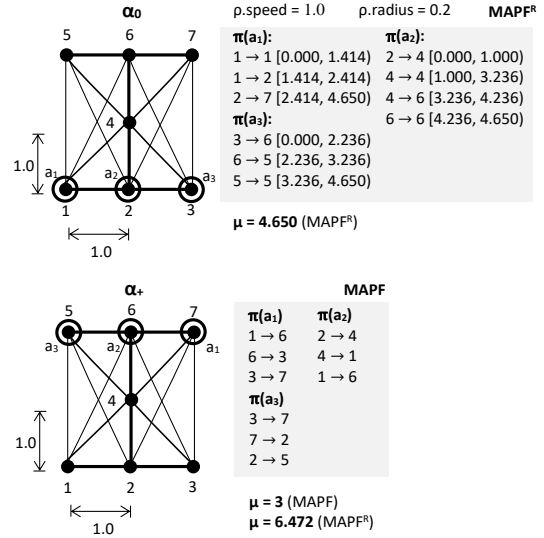
Figure 1: An example of MAPF R instance on a [3, 1, 3] -graph with three agents and its makespan optimal solution (an optimal solution of the corresponding standard MAPF is shown too).
