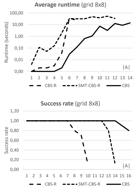
Figure 3: Comparison of CBS R and SMT-CBS R on 8 \times 8 grid with 2^k neighborhood ( k = 3 ).
