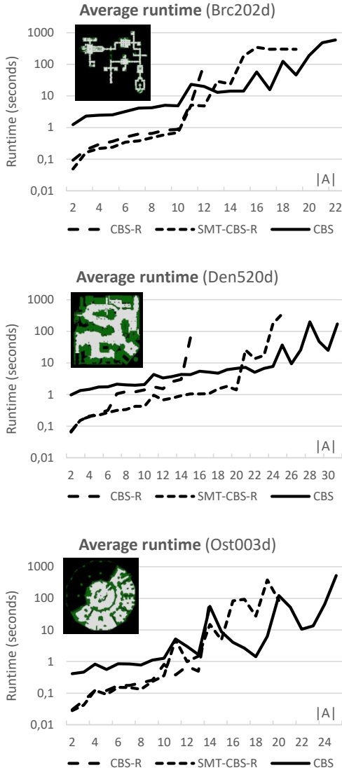
Figure 5: Comparison of \text{CBS}^{\mathcal{R}} and \text{SMT-CBS}^{\mathcal{R}} on game maps (Dragon Age) with 2^k neighborhood ( k = 3 ).
