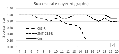
Figure 2: Comparison of CBS R and SMT-CBS R in terms of average runtime, makespan, and success rate on layered graphs. The standard CBS on the corresponding standard MAPF is shown too (times are in seconds). Makespan is shown for the case when the instance is interpreted as the standard MAPF and as MAPF R .
