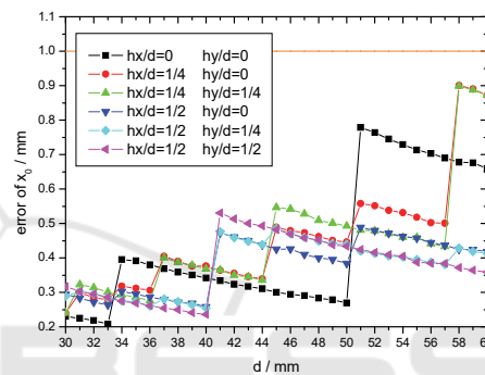
Figure 8: Fitting error of the facula center x_0 for two-dimensional simulation.
