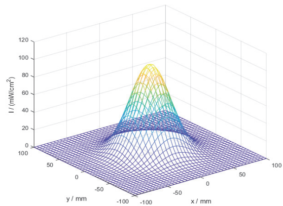
Figure 7: Result of two-dimensional fitting.
