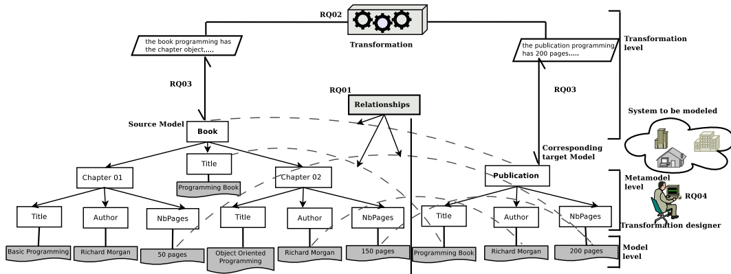
Figure 1: Model transformation problems.
