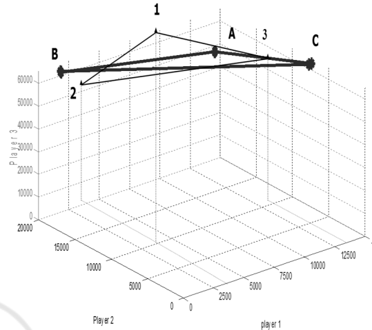
Figure 3: Socially Stable Core for a 5 bus TSC sharing game.
