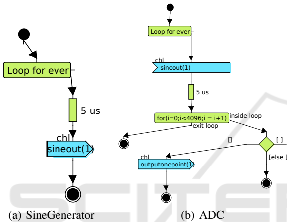
Figure 5: Activity diagrams of the analog modules.
