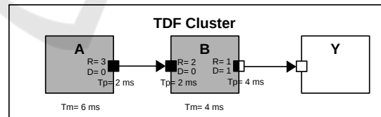
Figure 1: TDF cluster with two TDF and one DE module.
