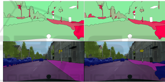
Figure 3: Prediction of the IoU values. The figure consists of ground truth (bottom left), predicted segments (bottom right), true IoU for the predicted segments (top left) and predicted IoU for the predicted segments (top right). In the top row, green color corresponds to high IoU values and red color to low ones, for the white regions there is no ground truth available.
