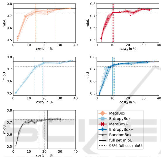
Figure 9: Results of single AL experiments (consisting of 3 runs each) for each AL method with the Deeplab model. Costs are given in terms of cost metric cost_A . In each plot, the single runs are given as dotted lines, the mean (over costs and mIoU) as a solid line. The vertical lines show where each run achieves 95% full set mIoU.
