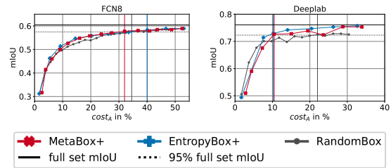
Figure 8: Results of the AL experiments for MetaBox+ and EntropyBox+. Costs are given in terms of cost metric cost_A . The vertical lines indicate where a corresponding method achieves 95% full set mIoU. Each method’s curve represents the mean over 3 runs.
