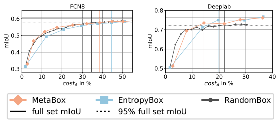
Figure 6: Results of the AL experiments for MetaBox, EntropyBox and RandomBox. Costs are given in terms of cost metric cost_A . The vertical lines indicate where a corresponding method achieves 95% full set mIoU. Each method’s curve represents the mean over 3 runs.
