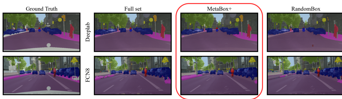
Figure 2: Segmentation results with our novel method MetaBox+ for two CNN models. With an annotation effort of only 10.47% for the Deeplab model (top) and 32.01% for the FCN8 model (bottom), we achieve 95% full set mIoU. Additionally, the segmentation results are shown when training the networks with the full dataset (Full set) and with a random selection strategy (RandomBox) producing the same annotation effort as MetaBox+. Annotation effort is stated in terms of a click based metric ( cost_A , Equation (10)).
