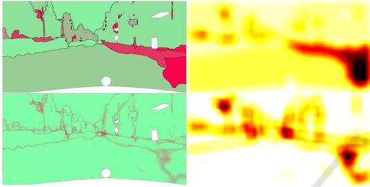
Figure 7: Comparison of query strategies based on MetaSeg and entropy. In the MetaSeg priority map (top left), low estimated IoU values are colored red and high ones green. Accordingly, in the entropy priority map (bottom left) low confidence is colored red and high confidence is colored green. The (line-wise) corresponding aggregations are given in the right hand column. The higher the priority, the darker the color.
