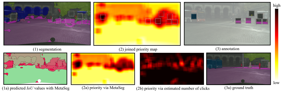
Figure 4: Visualisation of our AL method MetaBox+ at a specific AL iteration. The top row shows the segmentation (1), the joined priority map (2) and the acquired annotation (3). The joined priority map (2) is based on the priority via MetaSeg (2a) and the estimated number of clicks (2b). High values represent prioritized regions for labeling: in (2b) regions with low predicted IoU values are of interest in (2b) regions with low estimated clicks. (1a) shows the predicted IoU values via MetaSeg.
