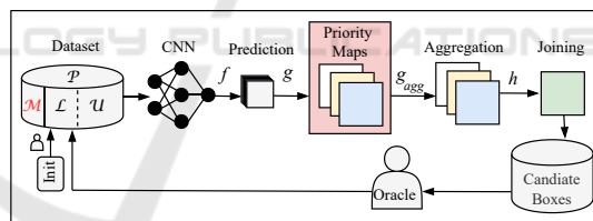
Figure 1: Illustration of the region based AL method. The red parts highlight the novel meta regression based ingredients: as query priority maps we use MetaSeg and the estimated number of clicks. Training of MetaSeg requires an additional small sample of data (fixed for the whole course of AL), indicated by \mathcal{M} \subset \mathcal{P} (in red color).
