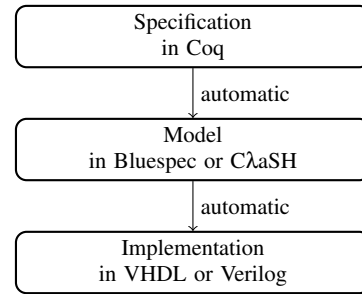
Figure 2: The correctness-oriented synthesis flows start with a specification using the proof assistant Coq. From the specification, a model in Bluespec (Kami) or ClaSH (Bornebusch et al., 2020) is extracted. The model is finally synthesized to an RTL implementation, e.g., in VHDL or Verilog.
