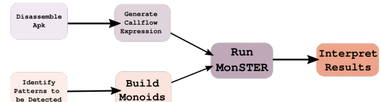
Figure 4: MonSTER workflow.
