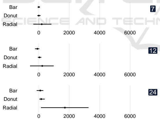
Figure 6: Difference between independent means of the small and large stimuli on the laptop screen for all chart types and individual data sizes . Error bars represent 95% Bootstrap confidence intervals (CIs).
