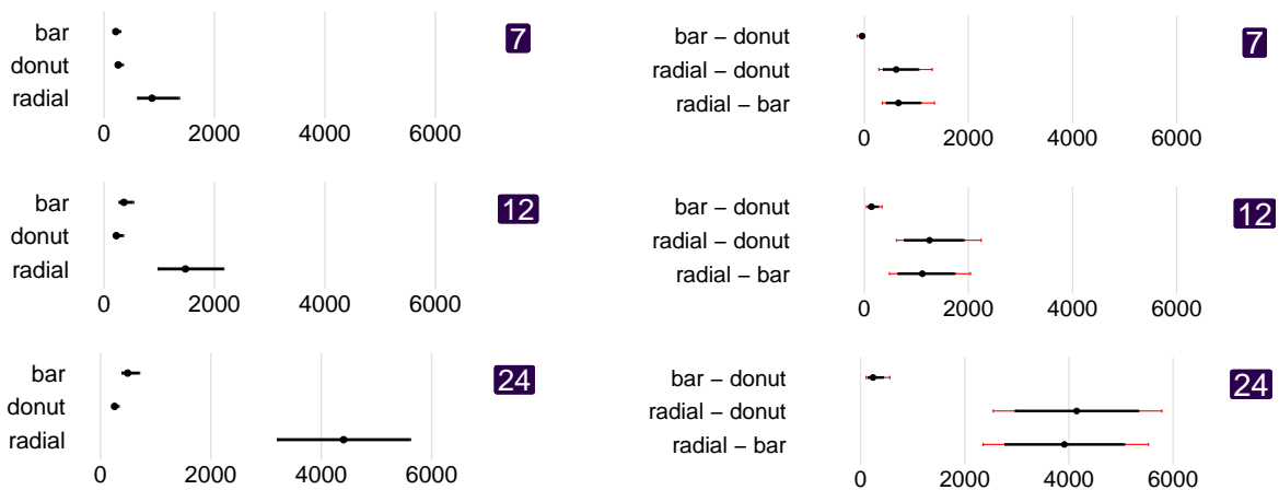
Figure 4: Results for the large stimuli displayed on the laptop screen (1280 px x 1280 px). Left: Average thresholds in milliseconds for each chart type and data size . Right: Pair-wise comparisons for each chart type and data size . Error bars represent 95% Bootstrap confidence intervals (CIs) adjusted for nine pairwise comparisons with Bonferroni correction.
