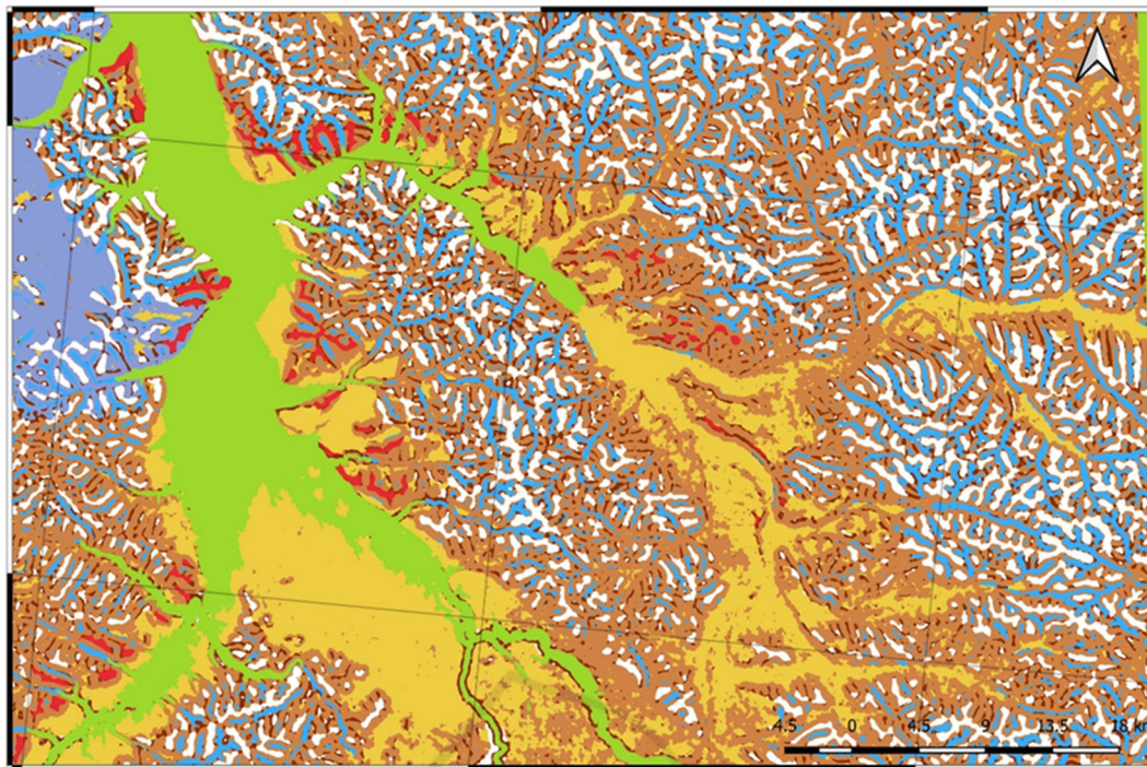
Figure 5: Permafrost landscape terrain type map by ASTER GDEM/ Scale 1:500 000.
