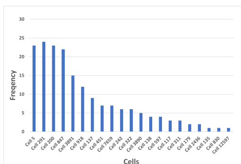
Figure 12: The number of times a cell has the maximum capacity in all the time slots.
