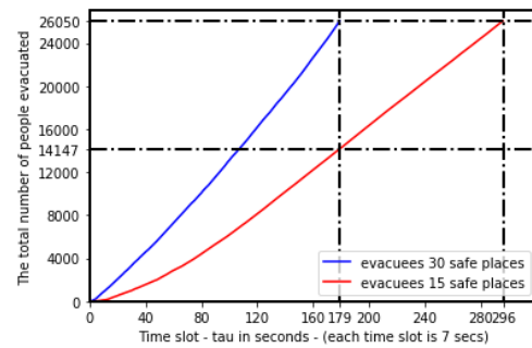
Figure 10: Total number of evacuees at each time slot for two scenarios - (a) 30 safe areas and (b) 15 safe places.
