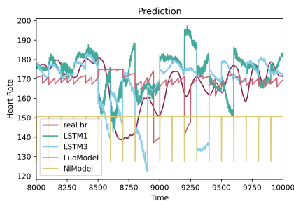
Figure 5: Comparison of Different Heart Rate Forecasting Models.
