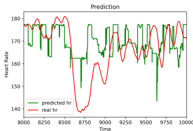
Figure 1: Heart Rate Forecasting of Random Forest Model.
