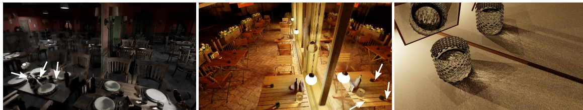
Figure 7: Our approach can be applied to more complex scenes (left image: 39 ms, path length of 7 segments; centre image: 46 ms, path length of 6 segments) and scales to more intricate caustics (right image, 1 s, path length of 6 segments; 175k spp for an equal quality path tracer). For the first two images, the main costs are path tracing (17–19 ms), light tracing (8–11 ms), and AS re-build (6 ms). All three images were rendered using our temporal version, and while the first two were filtered with SVGF, the last was accumulated over multiple frames.
