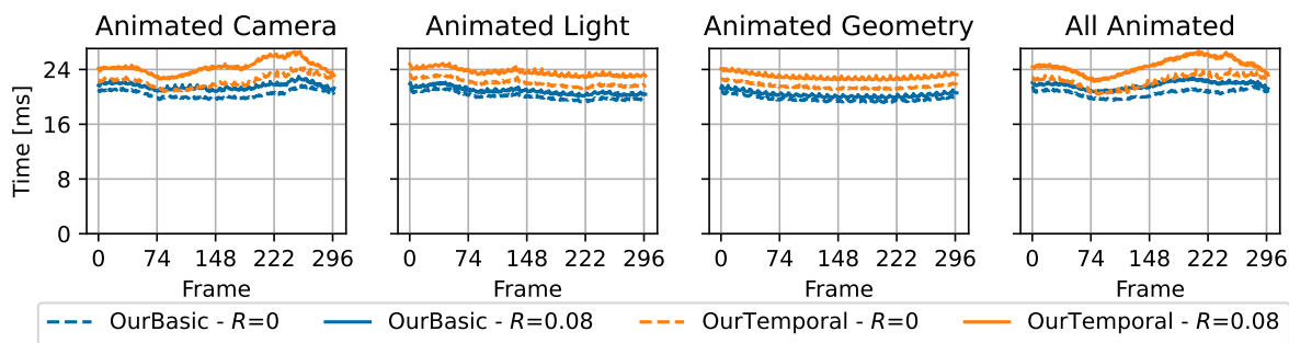
Figure 4: Measuring the total frame time taken by our basic and temporal algorithms for different types of animations. For comparison a path tracer at equal quality would require about 175 spp and take between 2.5 and 3 seconds; this was measured for equal FLIP-mean on AC@150 and AC@298.
