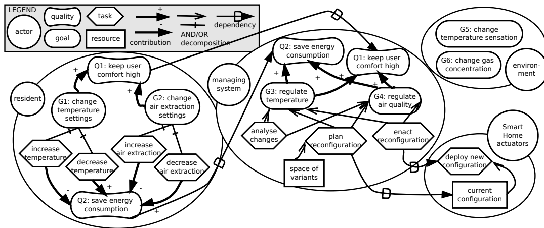
Figure 1: Goal-oriented model for the SHORE (Smart Home self-REconfiguration) approach.
