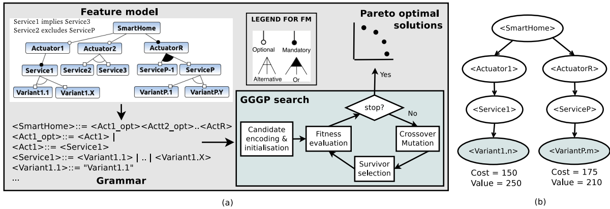
Figure 2: The SHORE approach: (a) the optimisation process, and (b) a candidate evaluation.
