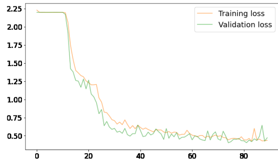
Figure 7: Loss learning curve.
