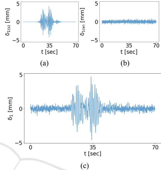
Figure 4: (a) example of seismic signal detected by sensor 1 during the simulation of seismic events; (b) example of environmental noise modelling traffic, temperature, pressure, rain, wind, and so on; (c) the integrated signal.
