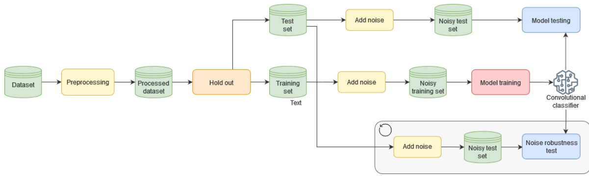
Figure 5: Data Pipeline.
