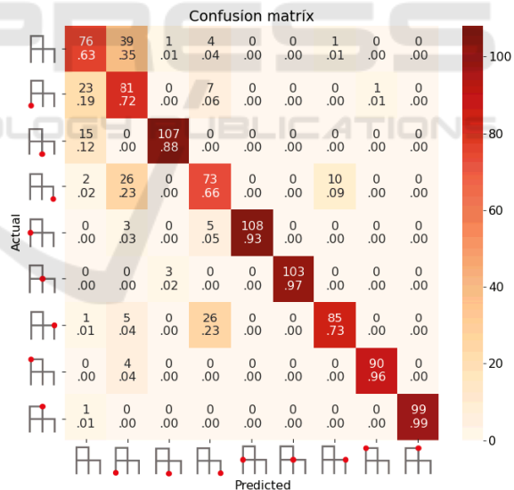
Figure 9: Confusion matrix on test set.
